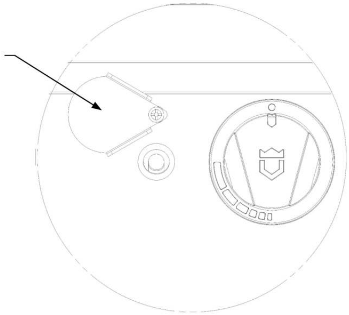
FIGURE 13. MANUAL LIGHTING
